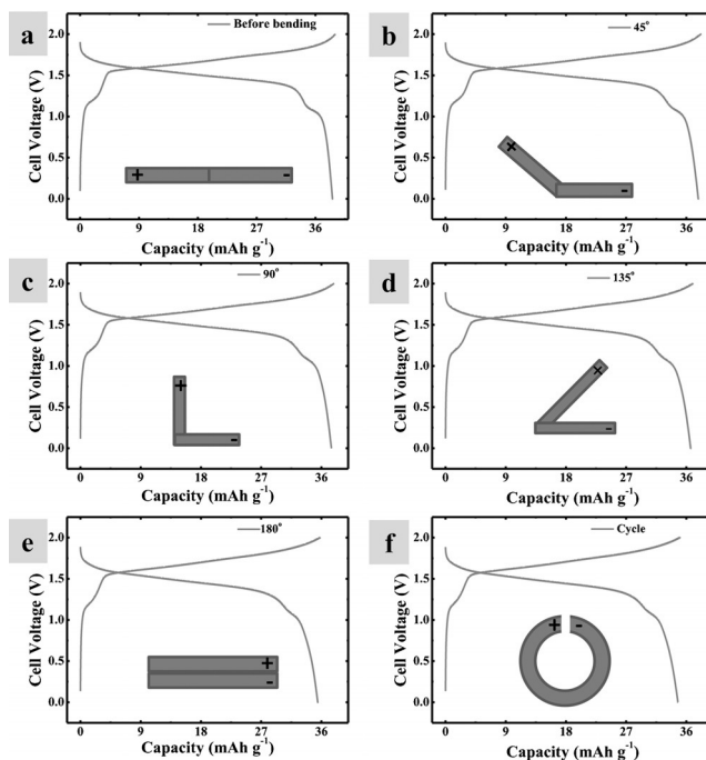
Figure 4. The performance of the flexible battery under different flexing angles. a) Flat state before bending; bended to (b) 45°; c) 90°; d) 135°; e) 180° and f) bended to a cycle.
